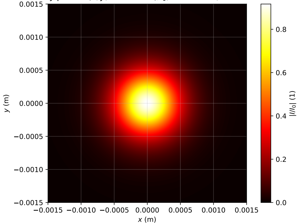
Intensity profile I(x, y, z = 2.707m)/I_0 , Pin=0.7Pcr, artificial time
